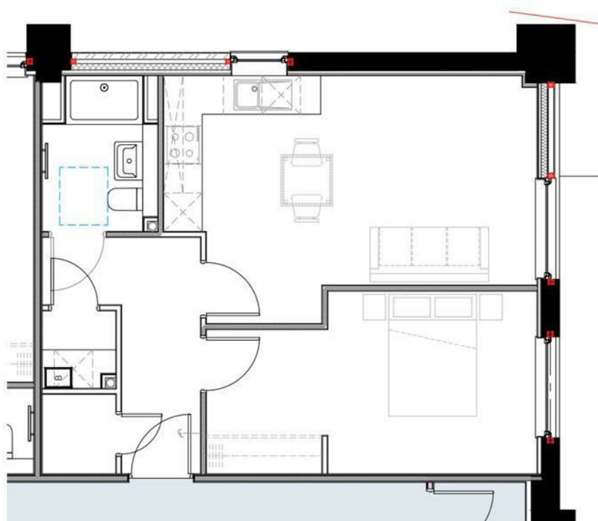
FLAT TYPE M ELECTRICAL SETTING OUT PLAN FLATS 8, 32, 56, 80 [AS DRAWN]. [SCALE 1:50 @A3]
